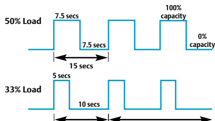
Digital Scroll Capacity Control Diagram
