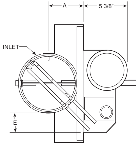
INLET VIEW
